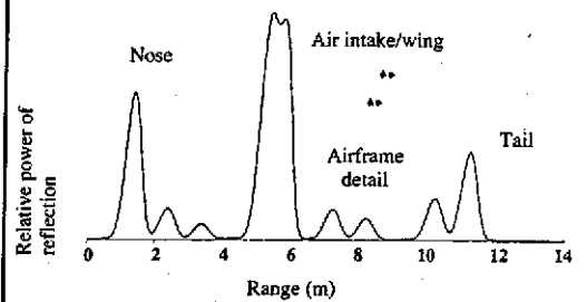
Representative compressed echo from aircraft
