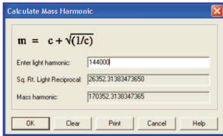
Figure 3: Calculate Mass Harmonic
