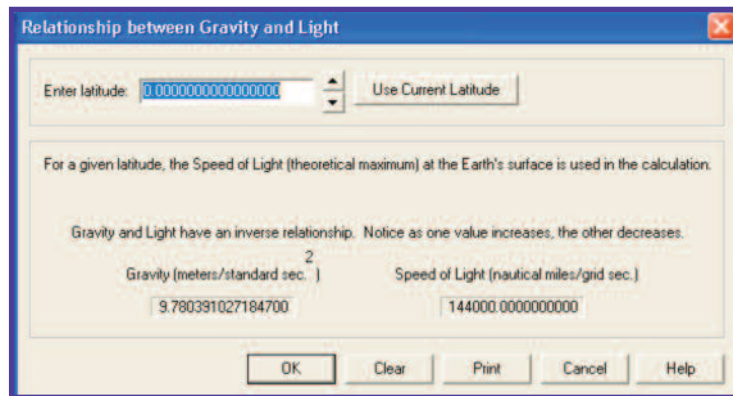
Figure 2: Relationship between Gravity and Light
