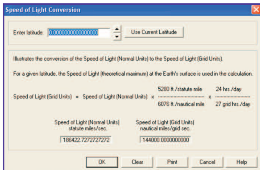
Figure 1: Speed of Light Conversion
