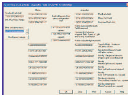
Figure 5: Harmonic Field to Latitude: Magnetic Field to Gravity Acceleration
