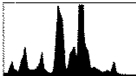
Tri-phosphor class II FL tube LUMILEX® PLUS CRI 85 / 3,000K (warm-white)
