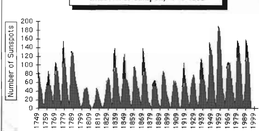
Chart No. 3: Sunspots, 1749-1993
