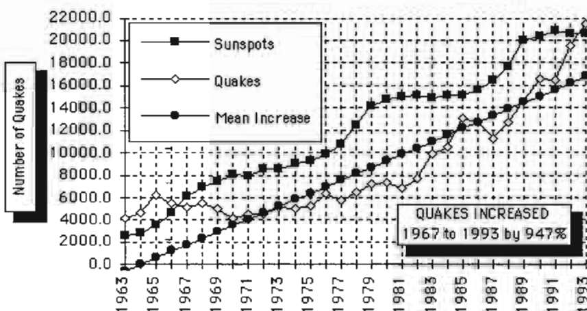
Chart No. 2: Global Earthquakes, 1963-1993 8
