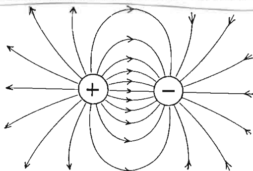
Ordinary electrical charges produce field lines that spread to infinity throughout the aether ('empty space').
