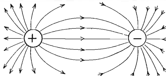
As the charges are moved apart, the connecting field-lines move apart and spread out unconstrained.
