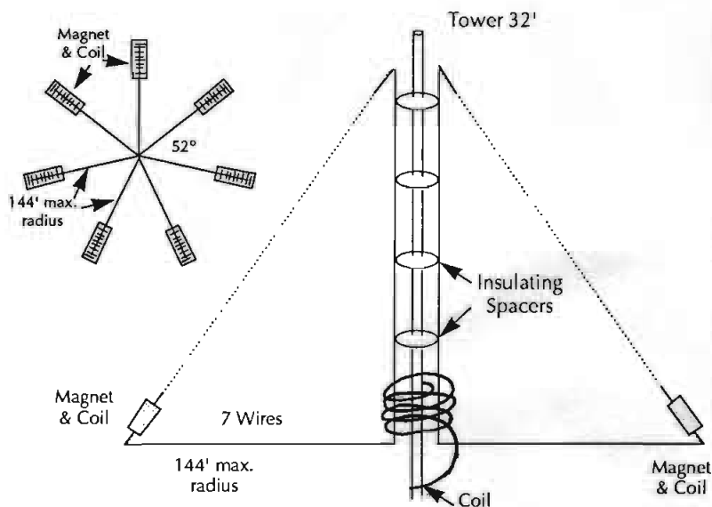
Figure 5: DeLand's "Frost-Guard Tower"
