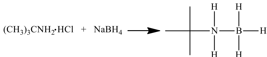
Figure 2. The Reaction to Produce tert -Butylamine: Borane Adduct.
