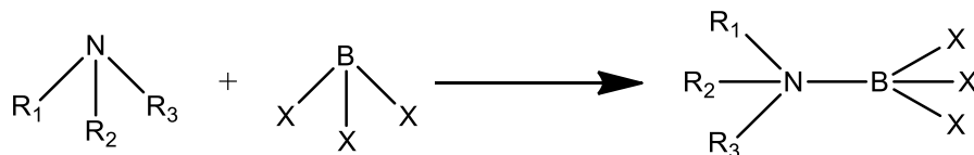
Figure 1. Reaction of an Amine with a Borane.
